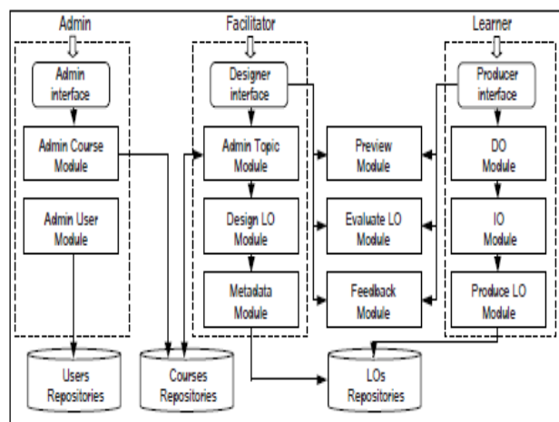
Figure 1. FLOM software architecture.
